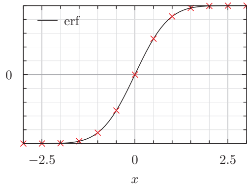
FIG. 1: The plot of the error function. The points indicate the values obtained by the erf function from stdlib .
