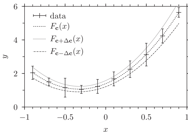
Figure 5.1: Ordinary least squares fit of F_{\mathbf{c}}(x) = c_1 + c_2x + c_3x^2 to a set of data. Shown are fits with optimal coefficients \mathbf{c} as well as with \mathbf{c} + \Delta \mathbf{c} and \mathbf{c} - \Delta \mathbf{c} .
