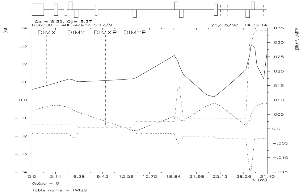
Figure 4: Beam size and divergence from the AD septum to the focal point of DEM for the measurement of vertical transverse emittance.
