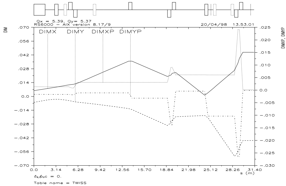
Figure 7: Beam size and divergence from the AD septum to the focal point of DEM for the large and parallel beam for antiproton channeling.
