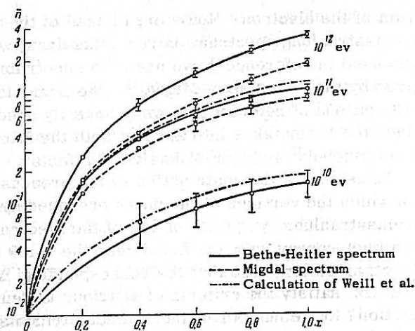
FIG. 2. Dependence of the average number of spurious tridents \bar{n} on the transverse distance \bar{x} (in radiation units) for various electron energies.
